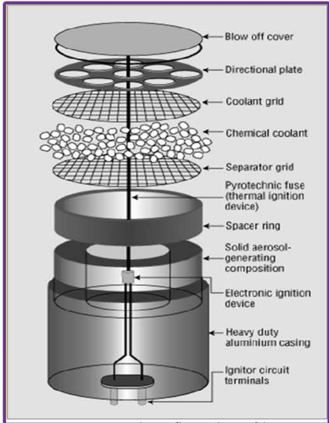
Explanation of the extinguishing device installation and its connection to the electrical current
